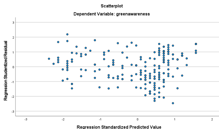
Figure 2. Scatter Plot Heteroscedasticity Test Results Source: SPSS Data Processing Results 2023
