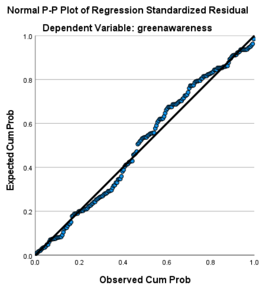
Figure 1. Normal P-Plot Test Results Source: SPSS Data Processing Results
