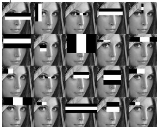
Gambar 1. Haar-cascade classifier
