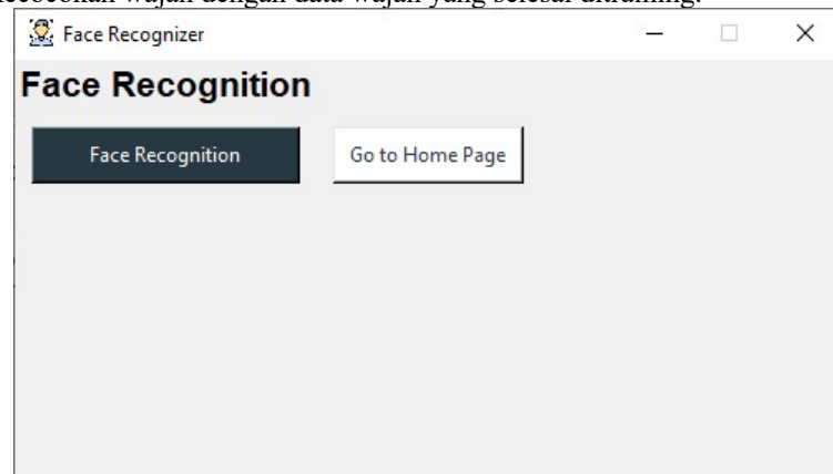
Gambar 9. Face Recognition
