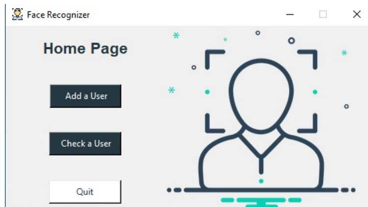
Gambar 6. Home page
